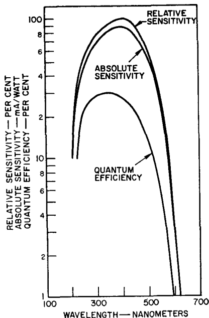
Fig. 33 — A set of typical spectral-response characteristics.
