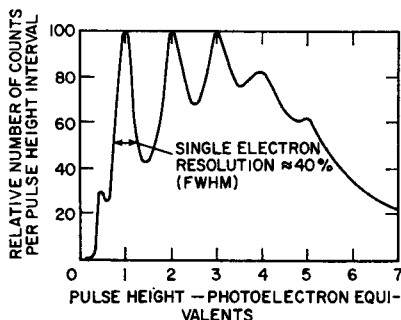
Fig. 77 — Single-electron distribution curve taken with a photomultiplier having a gallium phosphide first dynode.
