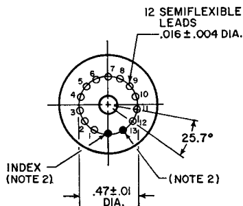
Fig. 25 — Lead-orientation diagram.
