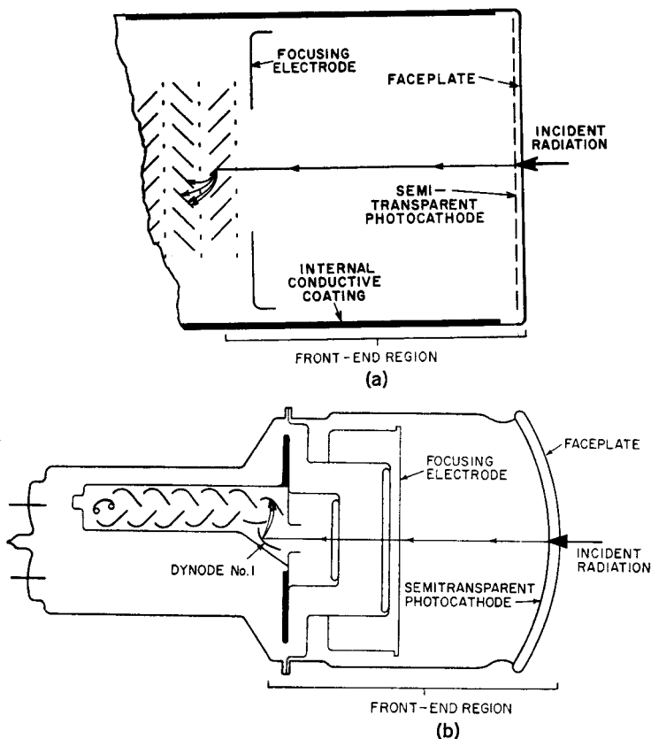
Fig. 12 — Front-end region of a photomultiplier with (a) a planar photocathode, and (b) a spherical photocathode.
