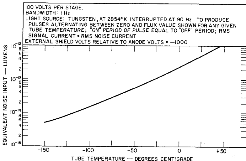
Fig. 37 — Equivalent noise input in lumens for a 1P21 photomultiplier as a function of temperature.
