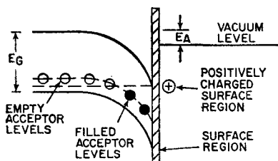
Fig. 3 — Semiconductor energy-band model showing negative electron affinity.
