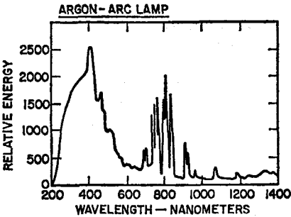
Fig. 101 — Typical spectral-emission curve for an argon-arc lamp.
