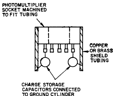
Fig. 90 — Tube socket mounted in copper or brass coaxial cylinder for negative-high-voltage applications.
