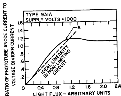
Fig. 83 — The relative response of a 931A photomultiplier as a function of the light flux using the circuit of Fig. 82 with equal stage voltage (at zero light level). Curve is taken from Fig. 2 of Ref. 1.
