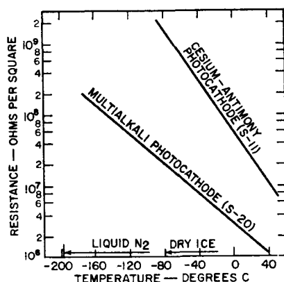
Fig. 28 — Resistance per square as a function of temperature for the cesium-antimony and the multialkali semitransparent photocathodes. These data were obtained with special tubes having connections to parallel conducting lines on the photocathode.
