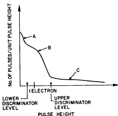
Fig. 76 — Dark-noise pulse-height-distribution spectrum.
