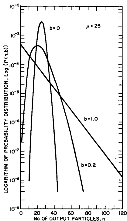
Fig. 58—Single-particle output distribution for a dynode displaying Polya statistics. A value of b = 1 gives a probably exponential distribution; b = 0 gives a Poisson distribution; b = 0.2 is intermediate between the two extreme values.
