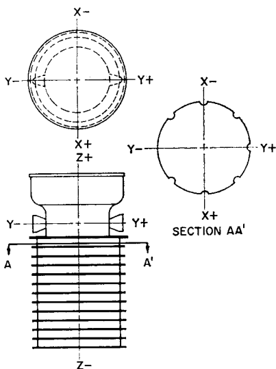
Fig. 23 — Test axes used in random-vibration and shock testing of stacked-ceramic photomultipliers.
