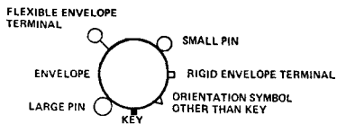
Key to Terminal Connections on Basing Diagrams.
