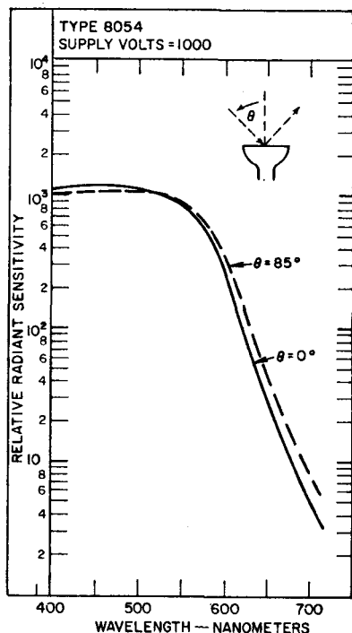
Fig. 47 — Spectral-response characteristics for a CsSb transmission-type photocathode for two different incident angles of radiation. The increased red response for the large angle of incidence may be explained in part by the increase in absorption caused by the longer path.
