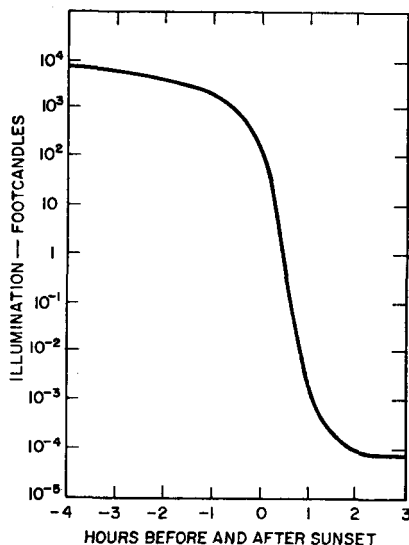
Fig. 94 — Natural illuminance on the earth for the hours immediately before and after sunset with a clear sky and no moon.
