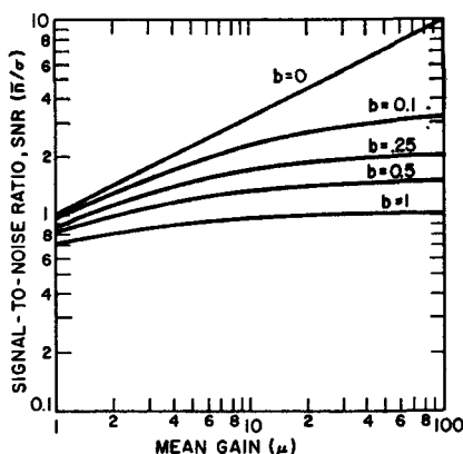
Fig. 59—A comparison of the SNR as a function of the mean value \mu for a number of Polya distributions. For Poisson statistics ( b = 0 ), the SNR increases as the square root of \mu . With 0 < b \leq 1 , the SNR approaches the square root of b^{-1} for large mean gains.
