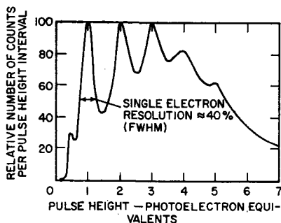
Fig. 54 — Typical photoelectron pulse-height spectrum for a photomultiplier having a GaP first dynode.
